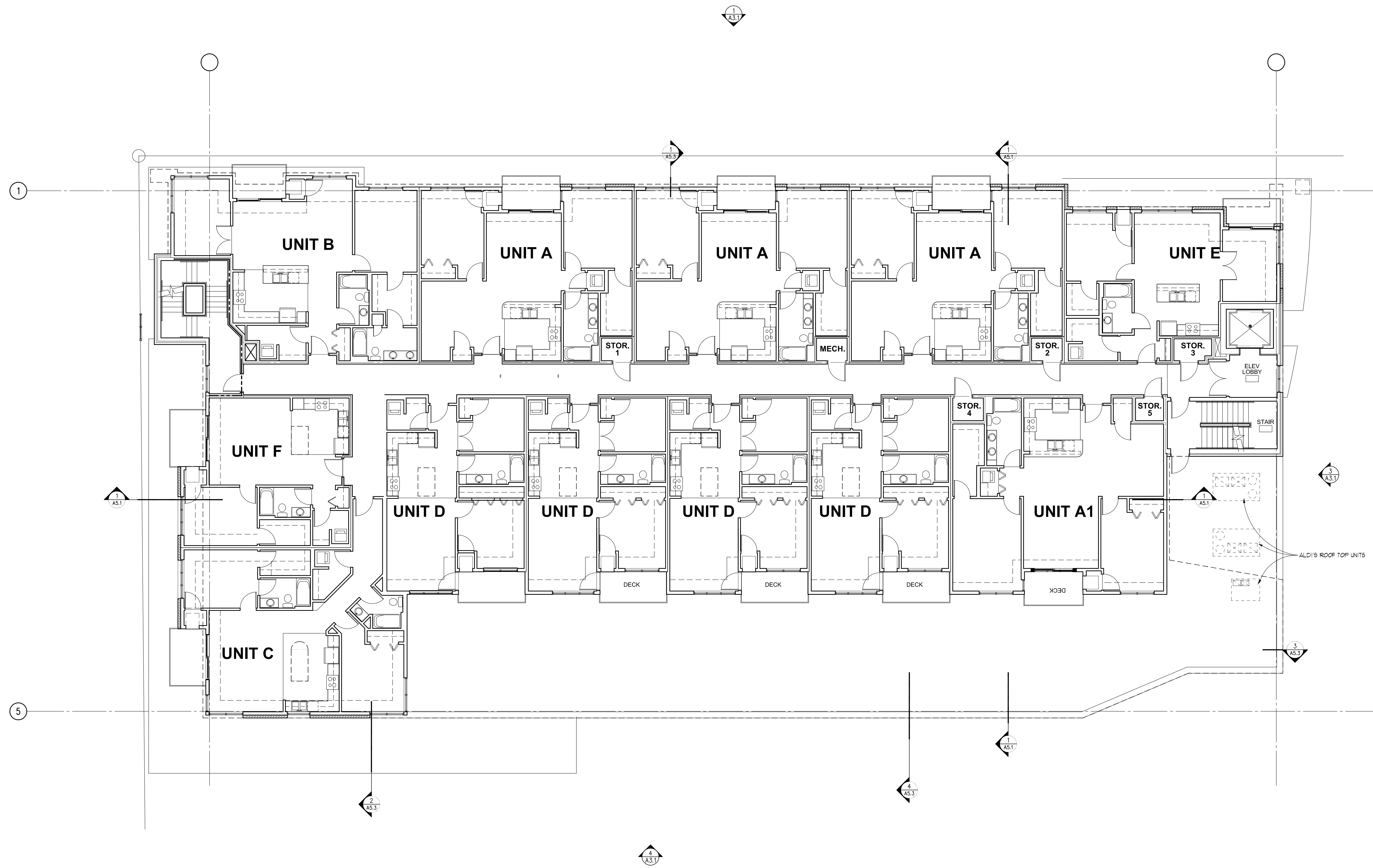
1 FIRST FLOOR HOUSING PLAN - (H1) A2.4 1/8"=1'-0"
